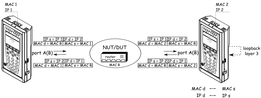
Figure 5.6. Connection scheme 2
