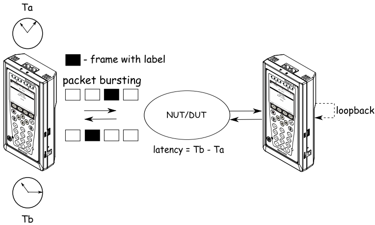
Figure 5.2. Latency
