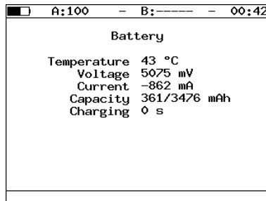
Figure 5.115. Battery screen
