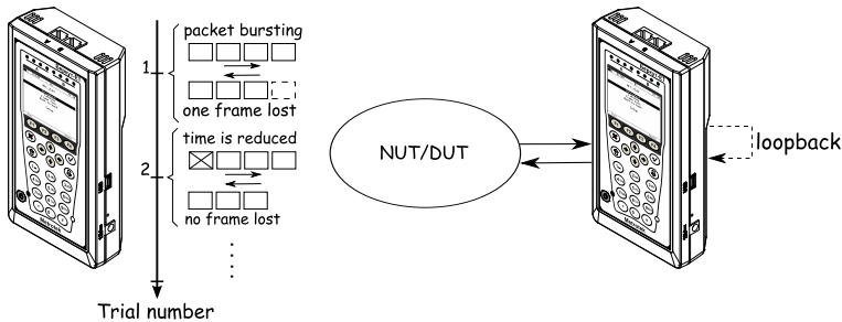
Figure 5.4. Back-to-Back
