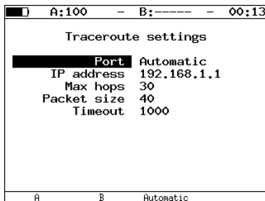
Figure 5.61. Traceroute settings
