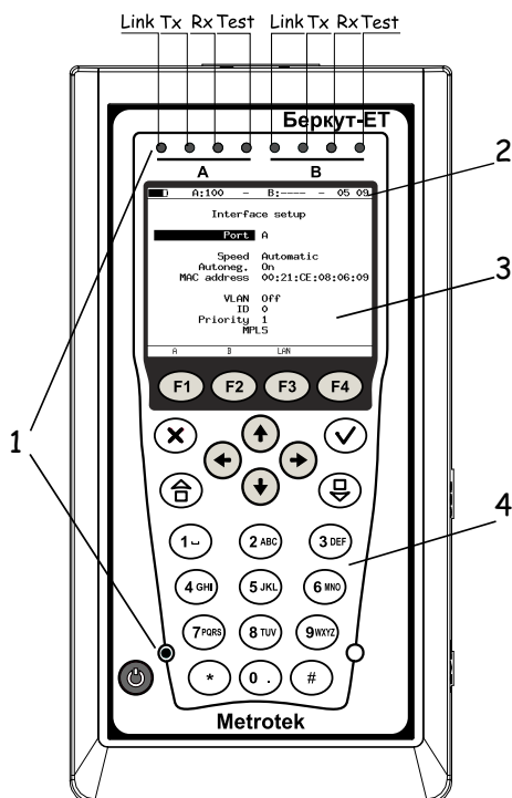
Figure 4.1. Front panel
