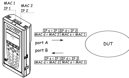
Figure 5.8. Connection scheme 4
